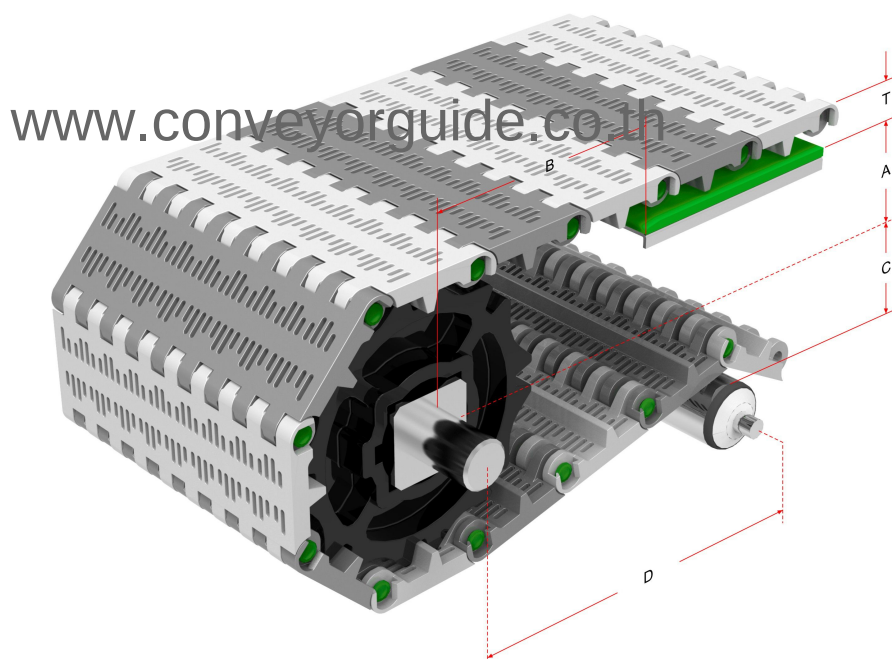
Conveyor Frame Dimensions
